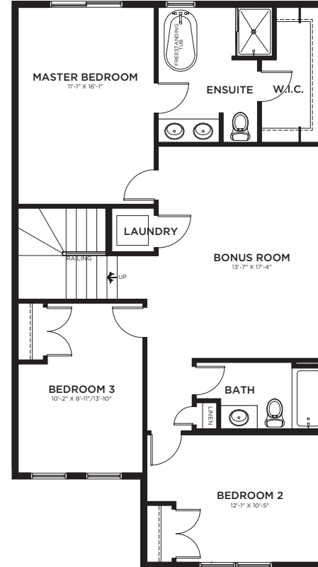
SECOND FLOOR PLAN 1066 SQ.FT. (NOT INCLUDING STAIRWELL)
